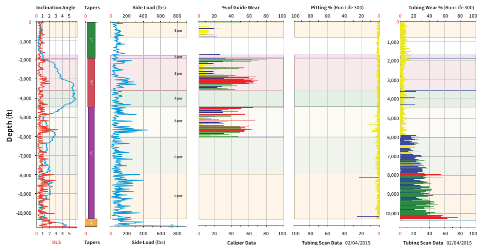
Combined WellTrak and RGAP Report Results displayed in an assortment of charts
