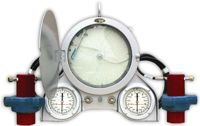
M365-Series Recorder with integral pressure gauges accepts dual inputs.
