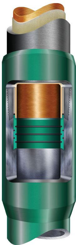
TK™-Ring – Accessory Interface
