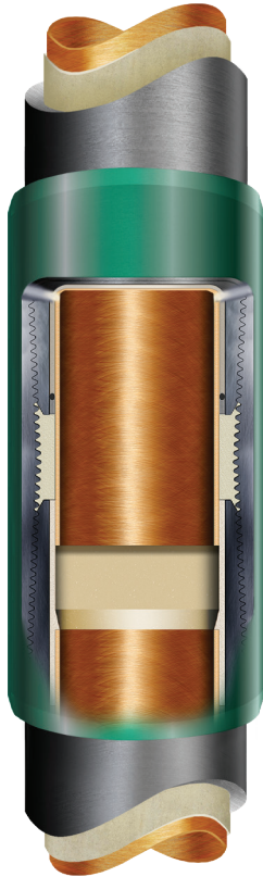
TK™-Fiberline I A ringless fiberglass lining system for API threads
