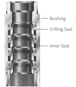
High Pressure Pack-off Assembly
